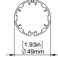
S45 HD Tube
