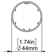
S45 STD Tube
