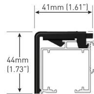
Spring Loaded Mounting Clip
