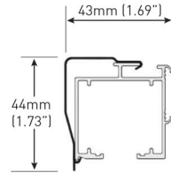
Low Profile Mounting Clip
